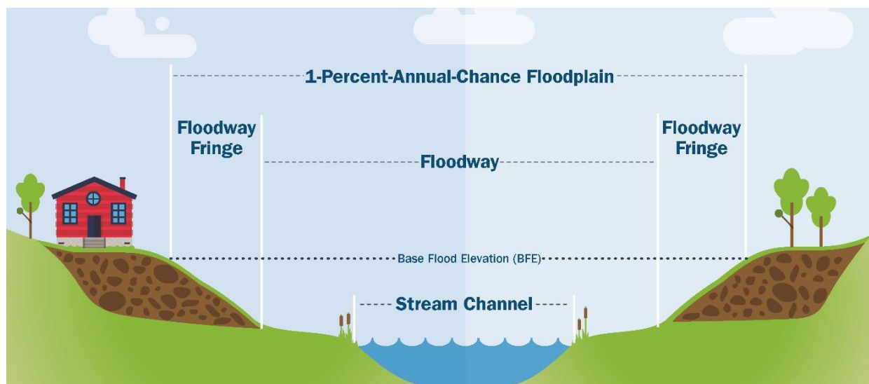
Figure 4.3.4-2 Diagram Identifying Special Flood Hazard Area, 1% Annual Chance (100-Year) Floodplain, Floodway and Flood fringe.
